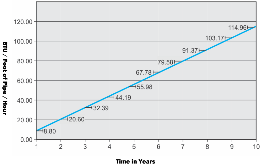
Estimated Heat Leak Performance - 1" IPS Foam Insulated
