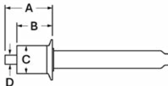
MALE BAYONET
